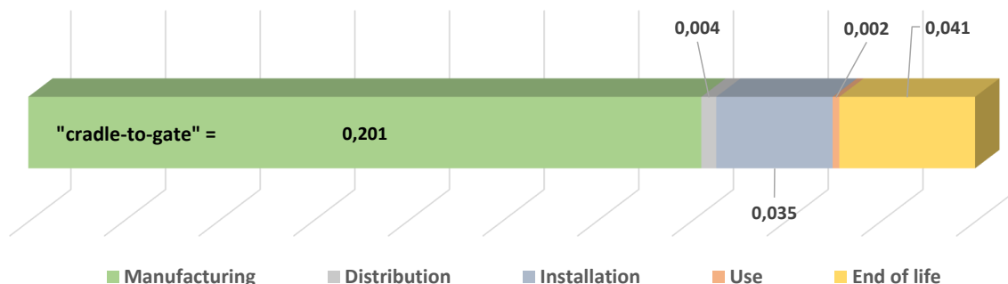
Climate change in kg CO 2 -eq for 1 meter of cable
