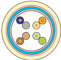
F/UTP Foiled / Unshielded Twisted Pair
