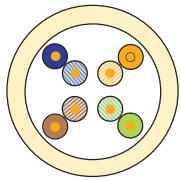
U/UTP Unshielded / Unshielded Twisted Pair
