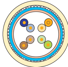
SF/UTP Shielded and Foiled / Unshielded Twisted Pair
