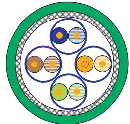
S/FTP Shielded / Foiled Twisted Pair
